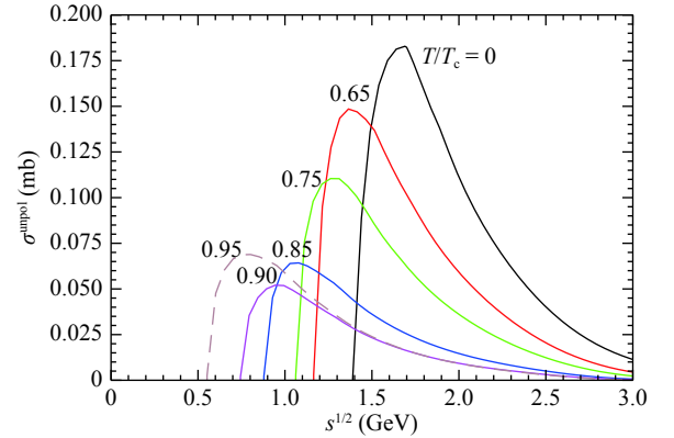
Fig. 7. (color online) Cross sections for \pi\pi \rightarrow K\bar{K}^* for I = 1 at various temperatures.
